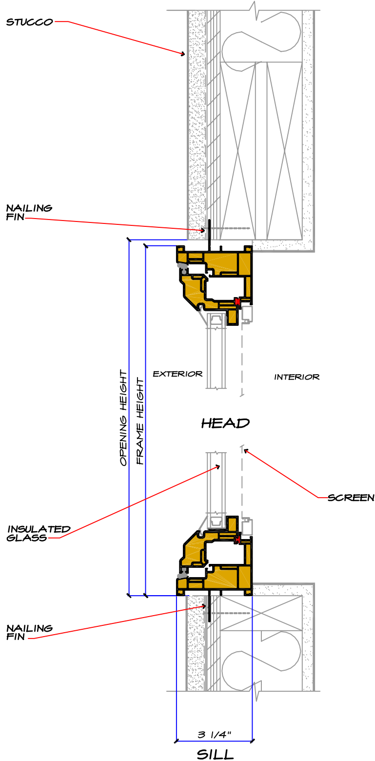
VERTICAL SECTION SCALE 3" = 1'-0"
