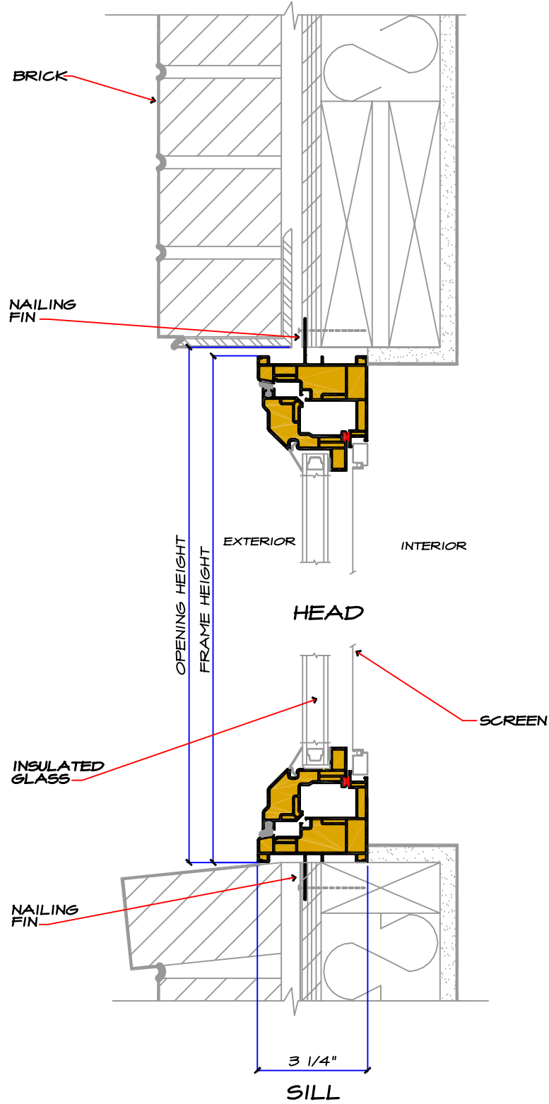
VERTICAL SECTION SCALE 3" = 1'-0"
