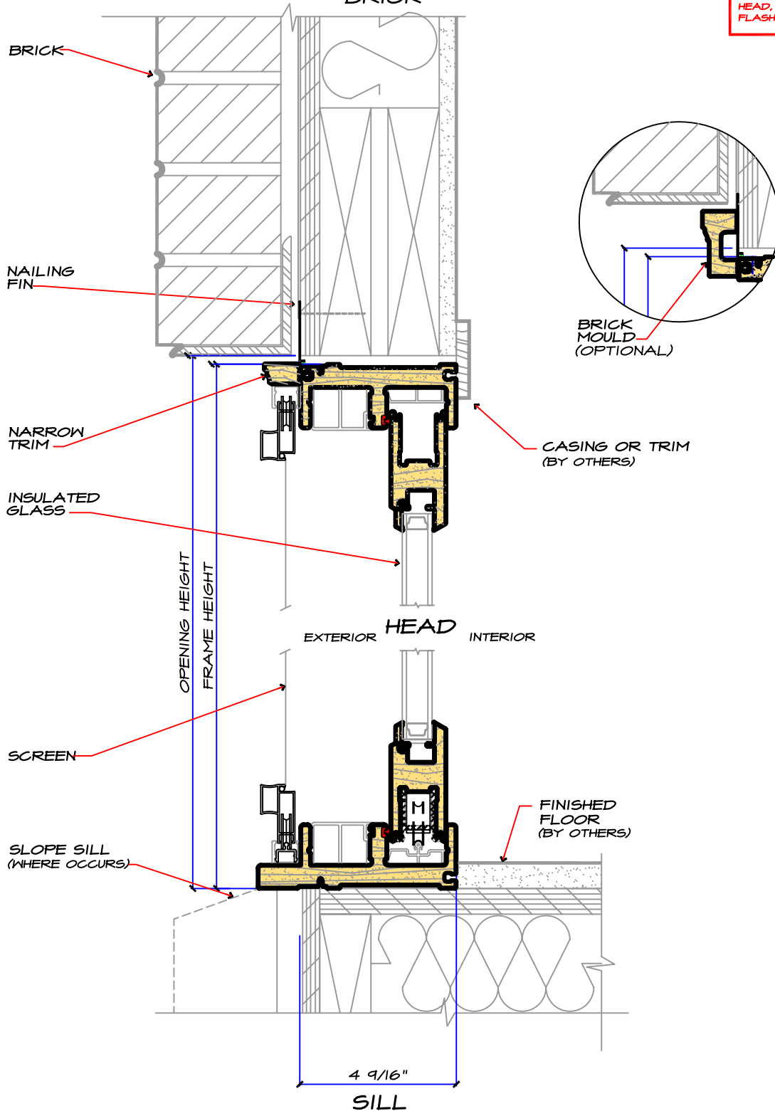
VERTICAL SECTION SCALE 3" = 1'-0"
