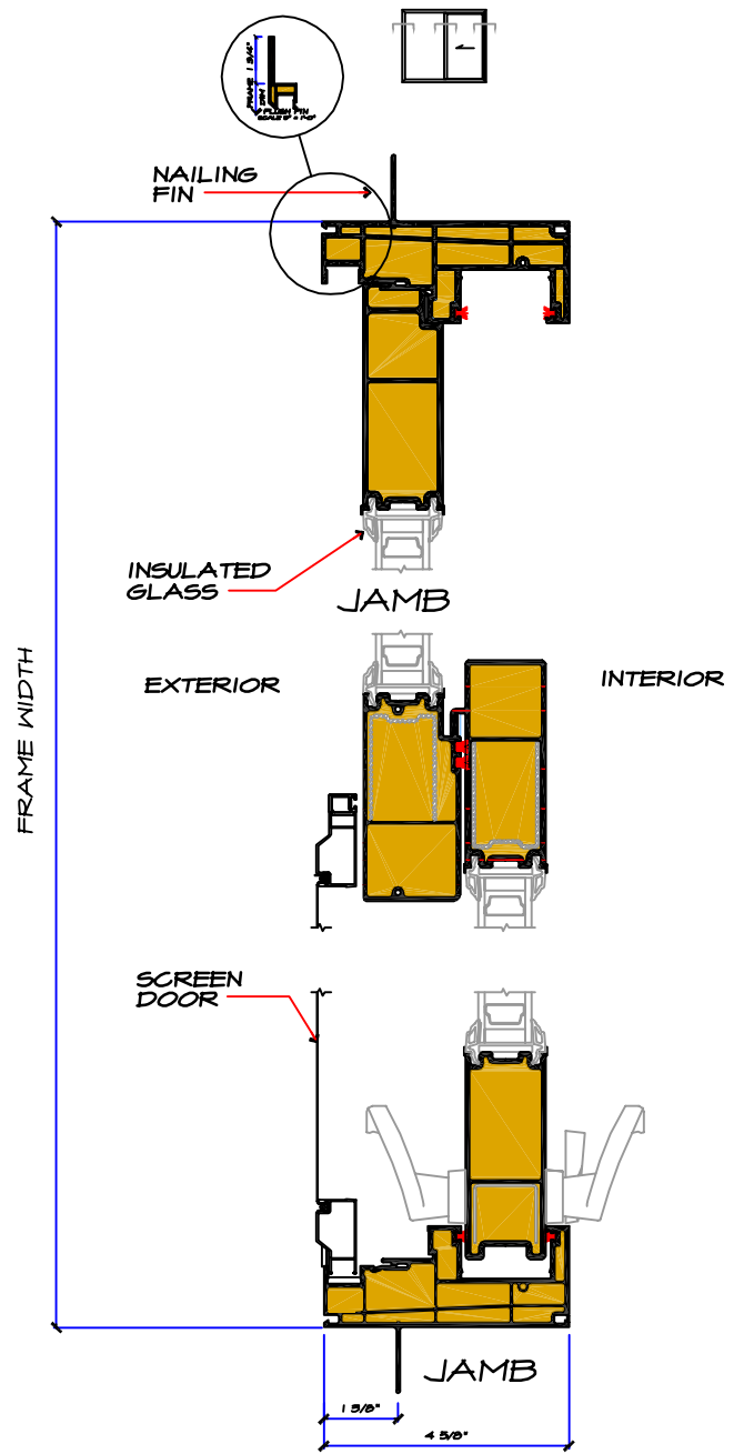
HORIZONTAL SECTION SCALE 3" = 1'-0"
